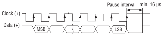
Figure 2. Timing Diagram
