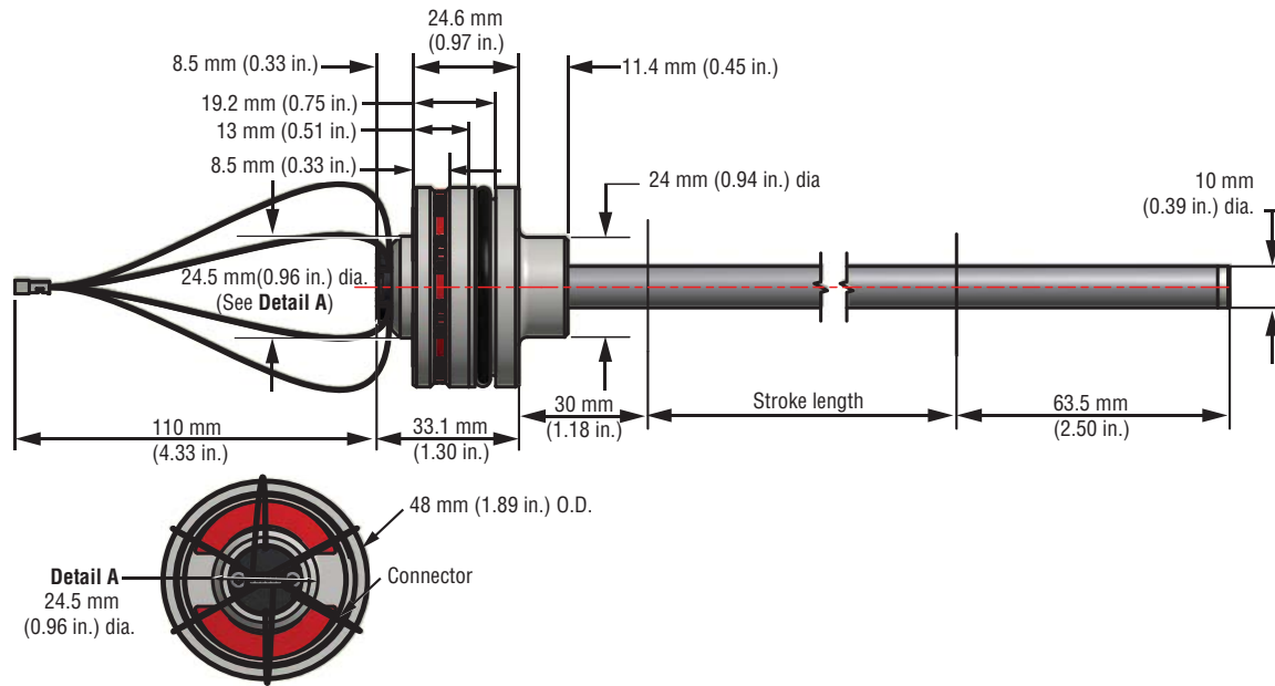
Figure 2. E-Series Model EE Sensor Component dimension reference
