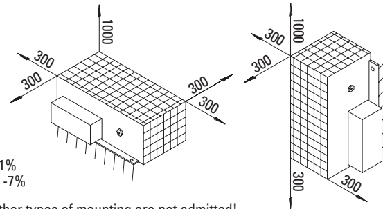
Admissible wall mounting Clamps down
