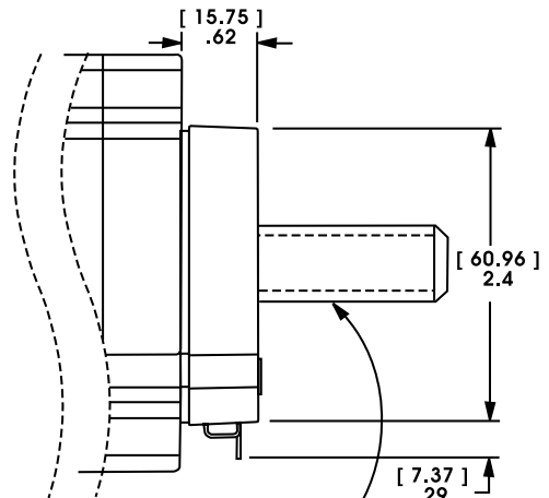
E6 87000 Series Size 34
