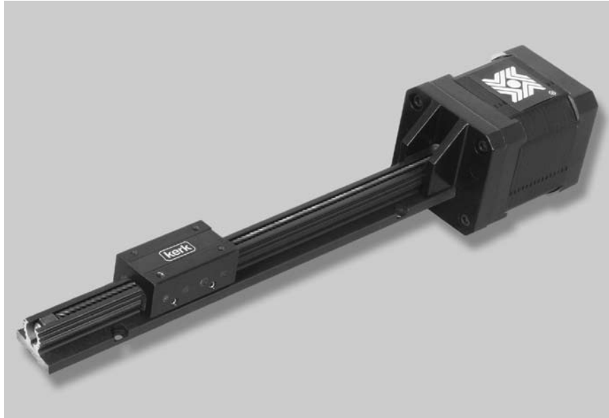
RGS04 with Size 17 Double Stack Hybrid Linear Stepper Motor
