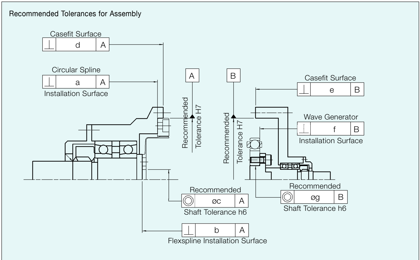
Tolerance for Assembly Table 11
