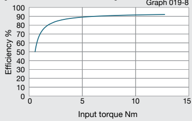
[Reduction ratio = 30, 35]
