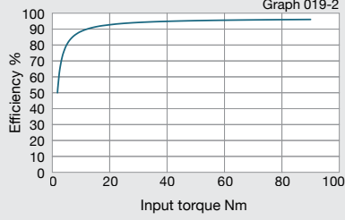
[Reduction ratio = 10]
