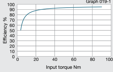
[Reduction ratio = 7]
