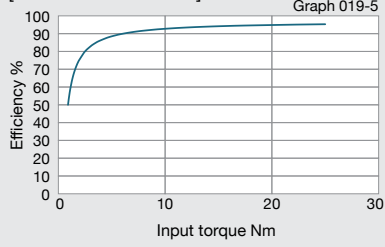
[Reduction ratio = 30, 35]
