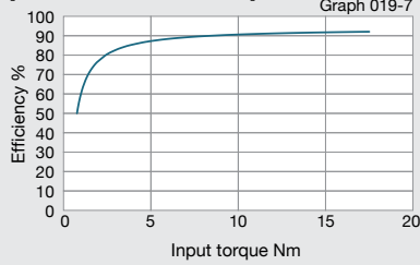
[Reduction ratio = 20, 25]
