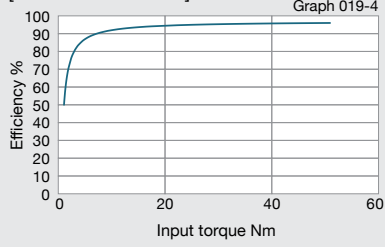
[Reduction ratio = 20, 25]
