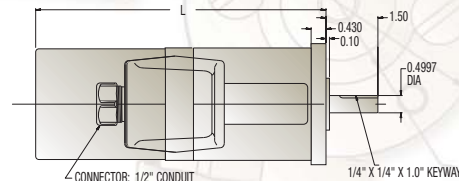
MOTOR TACHOMETER OPTIONS SHOWN: SQUARE MOUNTING, JUNCTION BOX, SEALED
