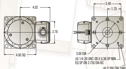
MOTOR TACHOMETER OPTIONS SHOWN: SQUARE MOUNTING, JUNCTION BOX, SEALED
