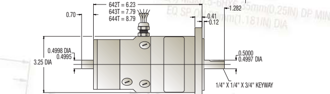
MOTOR TACHOMETER OPTIONS SHOWN: NEMA MOUNTING(42C), PG GLAND LEAD LENGTH (24" STD)
