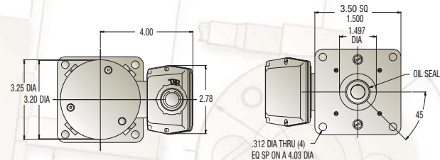
MOTOR TACHOMETER OPTIONS SHOWN: NEMA MOUNTING(42C), PG GLAND LEAD LENGTH (24" STD)
