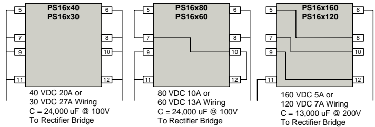
*Contact factory prior to rewiring transformer primary or secondary
