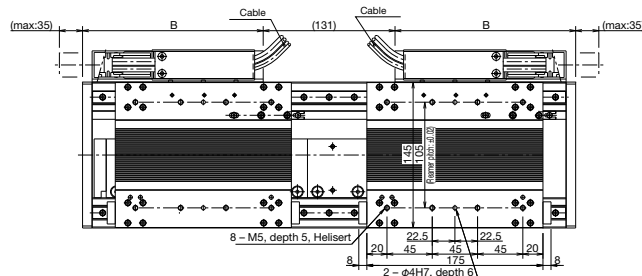
Detail view of base mount (S-1)
