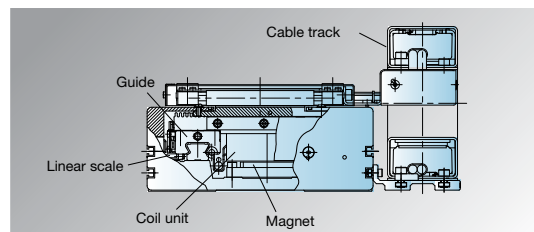
Section View of Large Type
