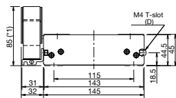
Detail view of base mount (S-1)
