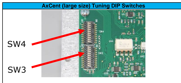
Figure 23 Tuning DIP Switches
