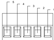
Existing analog motor/power connector
