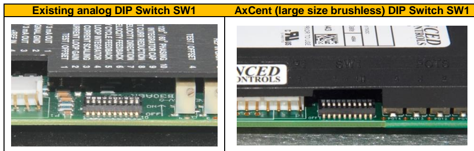
Figure 10 Configuration DIP Switch SW1
