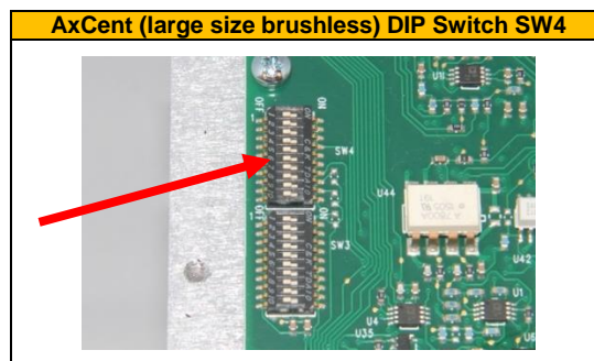
Figure 12 AxCent - DIP Switch SW4
